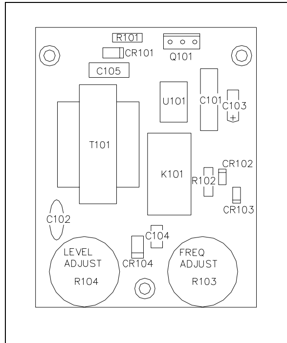
Figure 2. VLC PCBA Component Location
