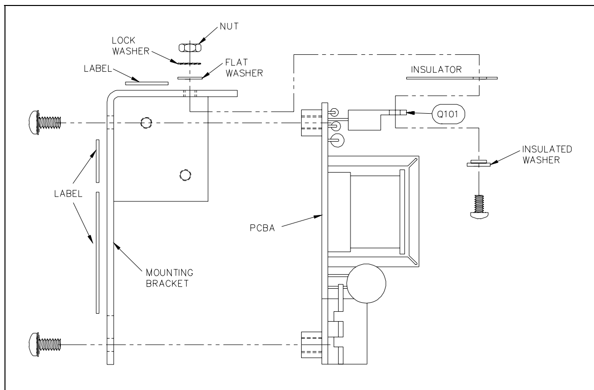
Figure 1. VLC Assembly
